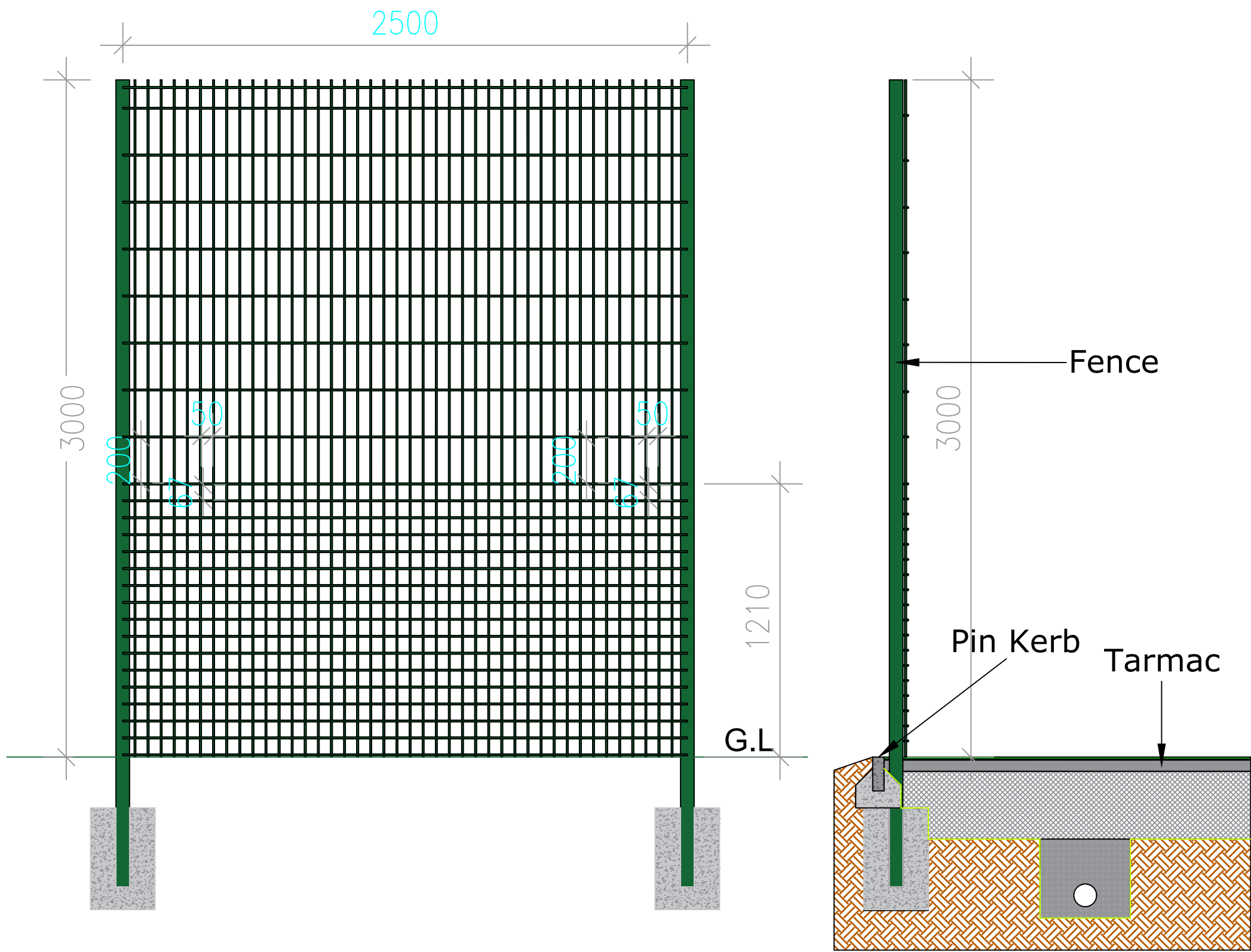
Typical Muga Fence Detail - Scale 1:20
