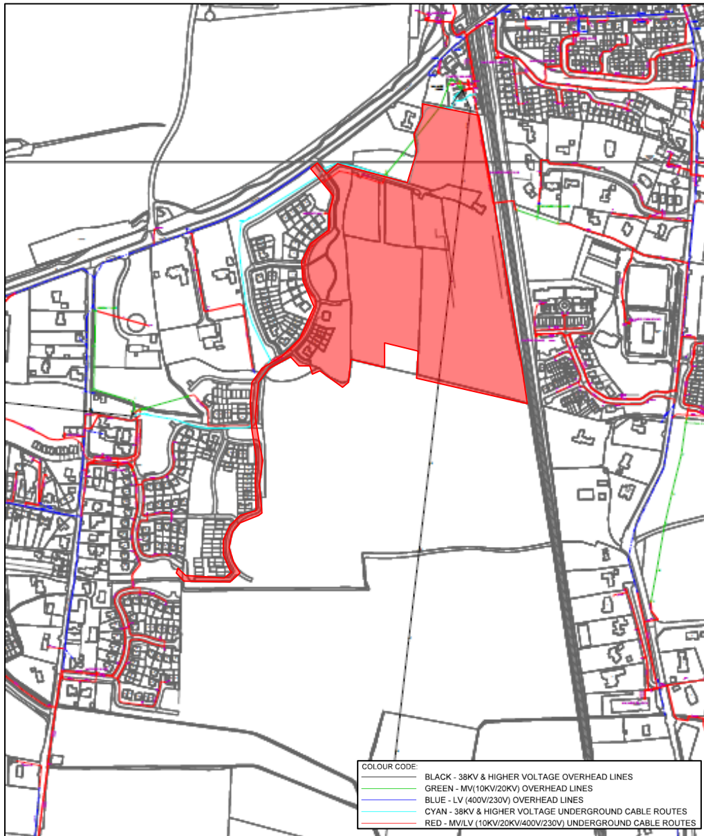
Figure 12.2 | Existing ESB Network Layout
