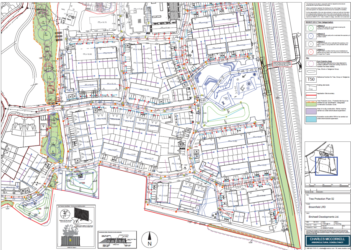
Figure 5.17. Tree protection Drawing (Mc Corkell (2024)).
